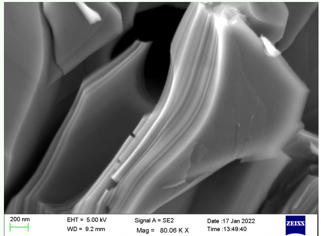
Fig.1 SEM image of the Ti_3AlC_2 MAX phase synthesised at 1400 °C
