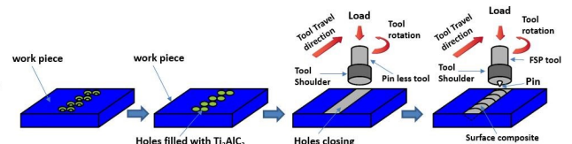
Fig.2 Schematic of the FSP process to form surface MMCs
