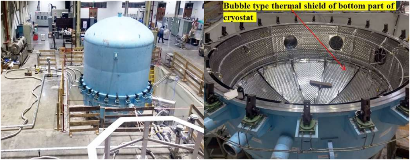
Figure A.4.1.3. (a) Integrated Magnet Test Facility (MTF) operating at 4.5 K and currents upto 10 kA. This joint is of practical importance because it can be integrated in the limited space available near Nb 3 Sn CICC-based superconducting magnets
