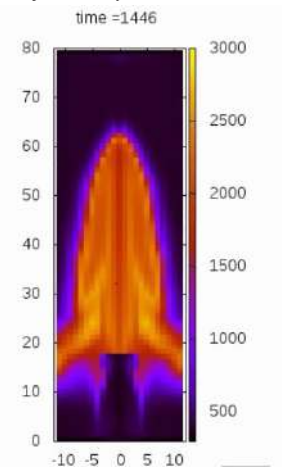
Figure A.5.1.2g E-field profile of the Passive Active Multi-junction (PAM) launcher using CST for Aditya-U Tokamak
