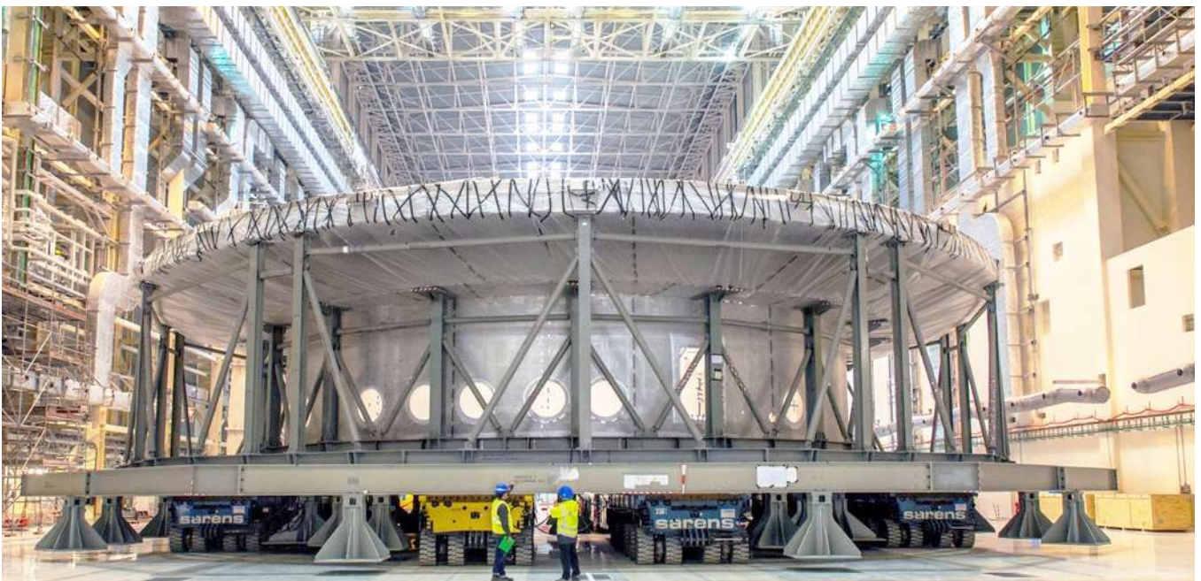
Figure B.3 Base Section Moved from Cryostat workshop to assembly Hall building. Installation in the tokamak pit and welding activities to commence soon
