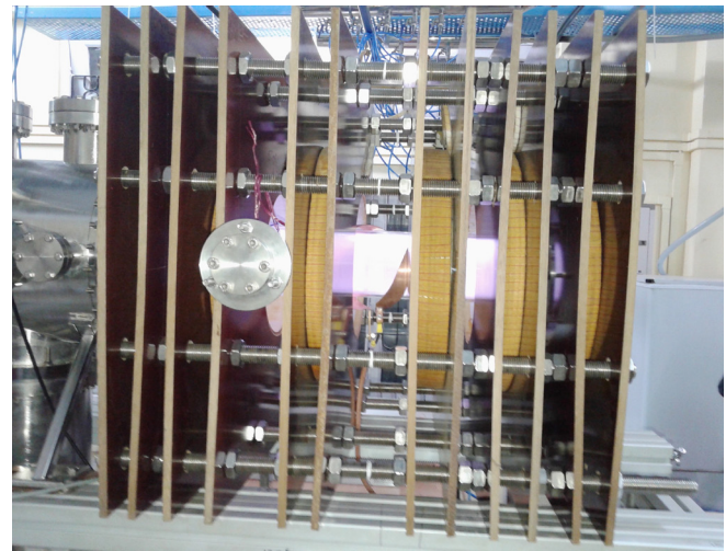
Figure A.1.8 Argon plasma produced in the HeliPS system
