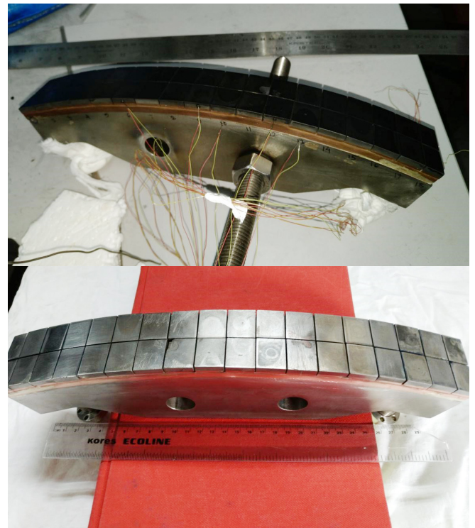
Figure A.2.4 Fabricated DOME successfully tested up to 5MW/m 2 using HHFTF
