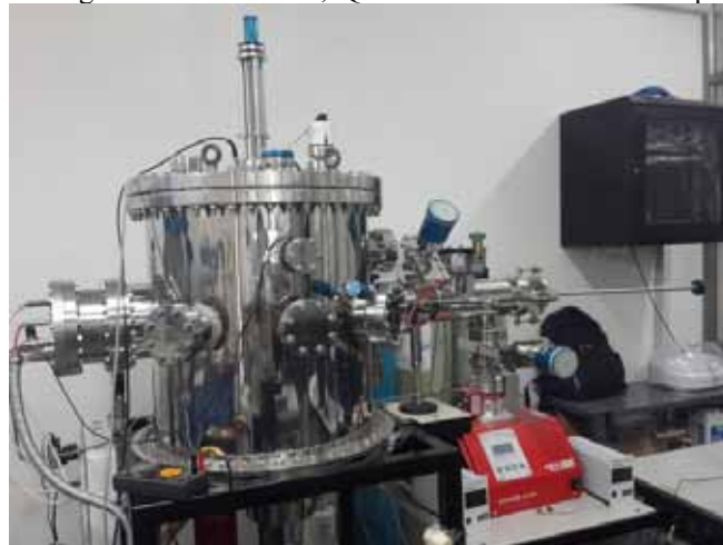
Figure B.1.3 Developed Ion beam facility
