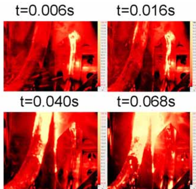
Figure A.1.1.3 Thermographic frame sequences -shot# 21655
