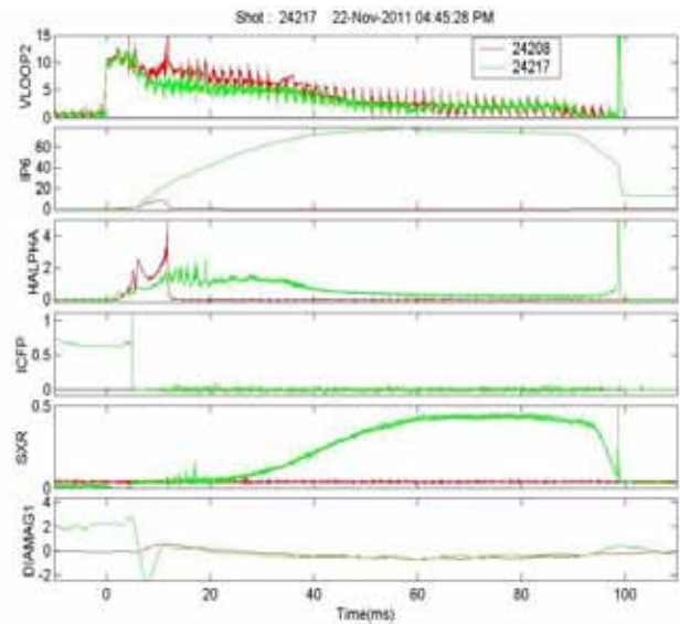
Figure-A.1.1.3.3 Left - time traces of plasma current, applied loop voltage, ICRF pulse and measured density . Right - two similar shots one is with ICRH pre-ionization (green) and other without it (red). The figure clearly shows a normal plasma current ramp up at low loop voltage with ICRH assistance.
