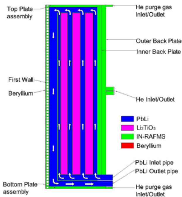
Figure A.2.3.1 Schematic view of Indian LLCB TBM
